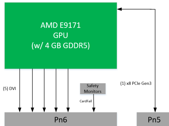
Figure 1: GPM0002 XMC Module Block Diagram
